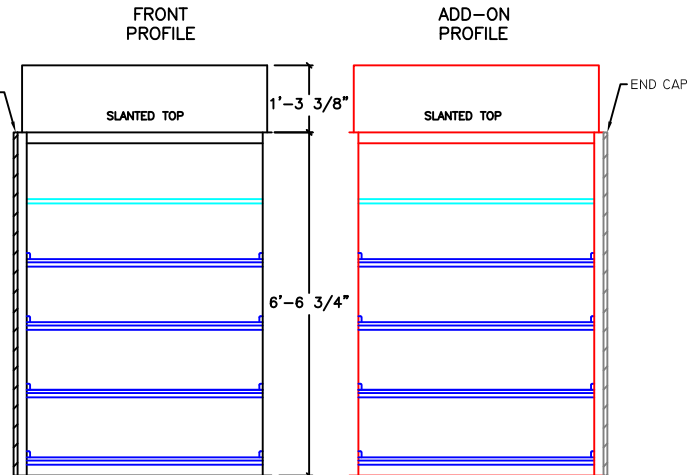
TYPICAL SHELF CONFIGURATION
