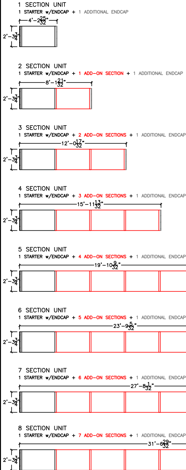
TOP VIEW - FOOTPRINT
