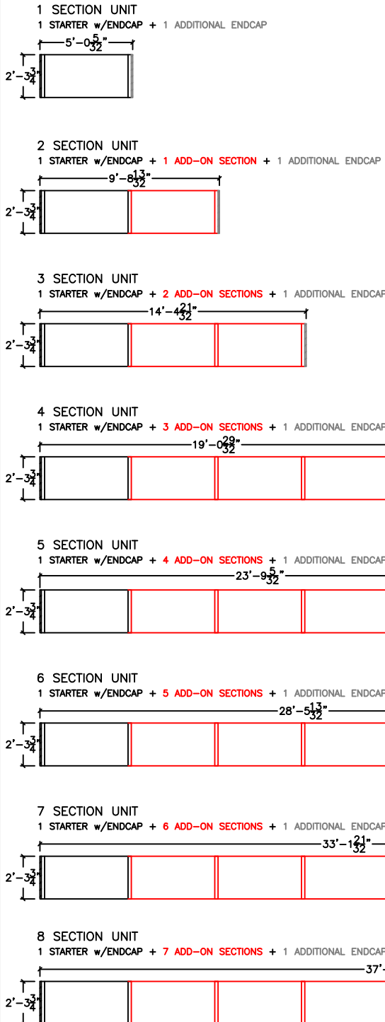
TOP VIEW - FOOTPRINT
