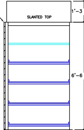
FRONT PROFILE
